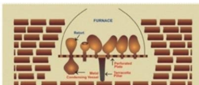
Graphical representation of the furnace
